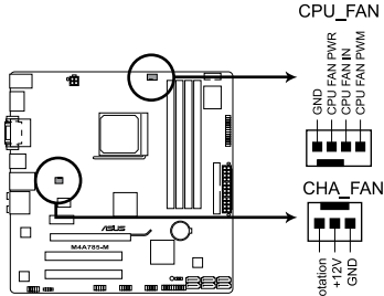
M4A785-M fan connectors
