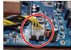
Plugged from an 8-pin EPS12V power.
