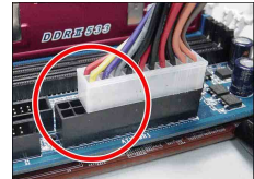
Plugged from a 20-pin ATX12V power.
