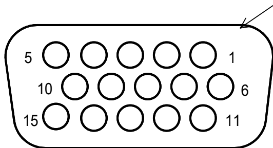
D-sub connector
