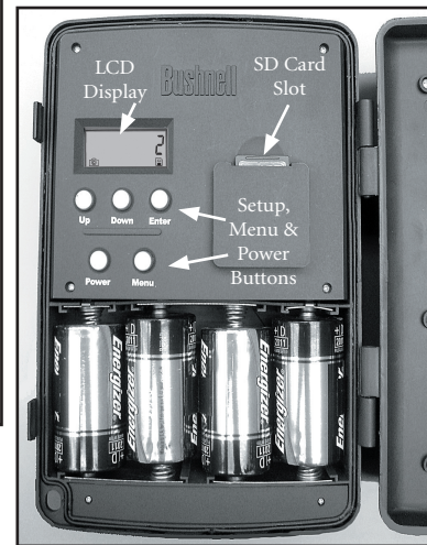
Control Panel Inside Front
