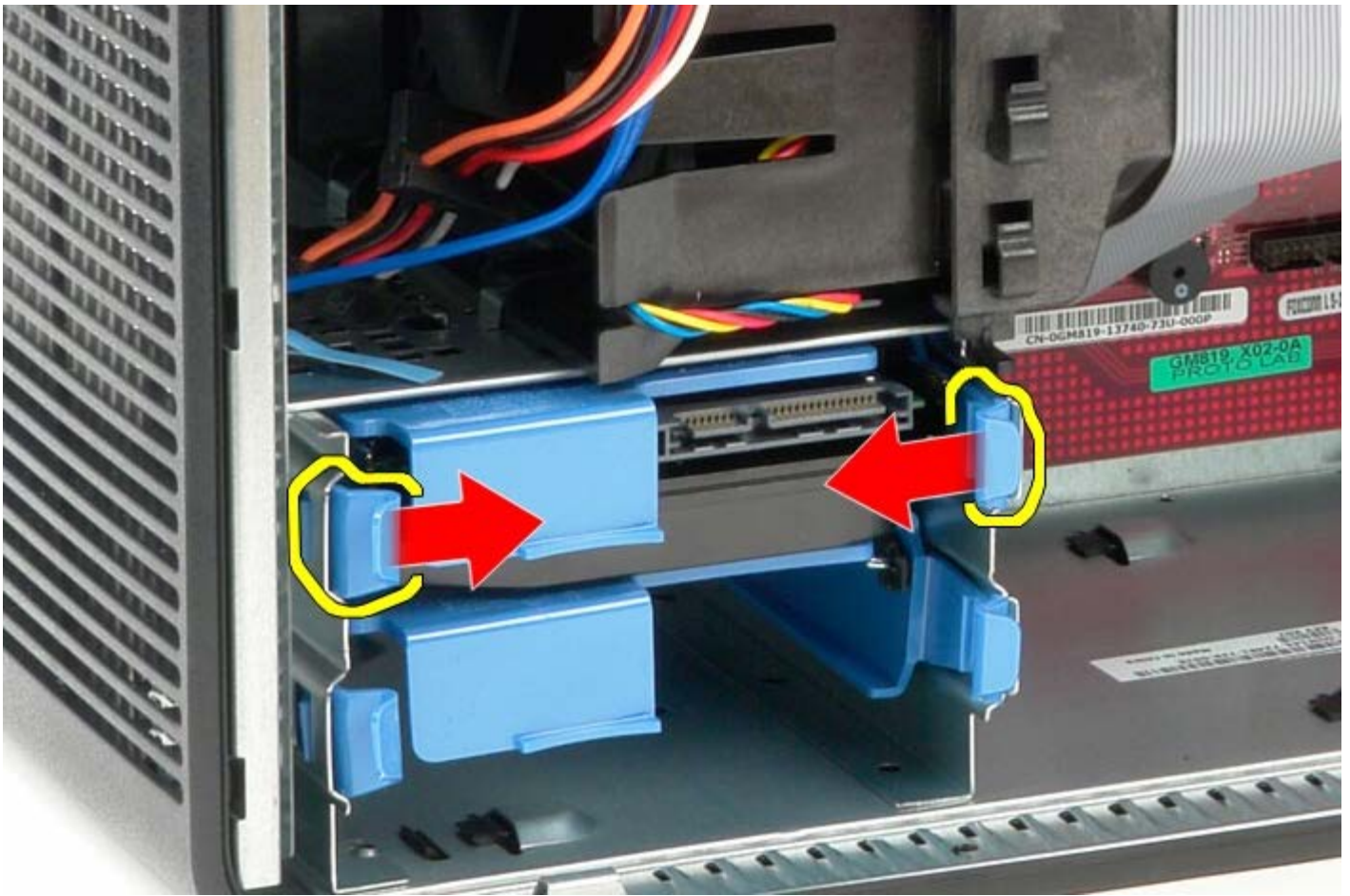
6. Slide the hard drive out of the computer.
