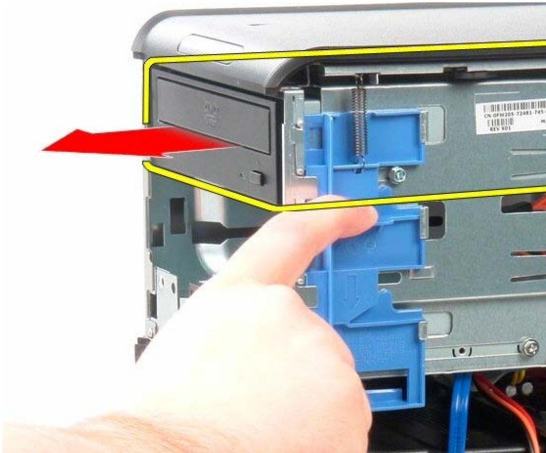
6. Slide the optical drive out of the system.
