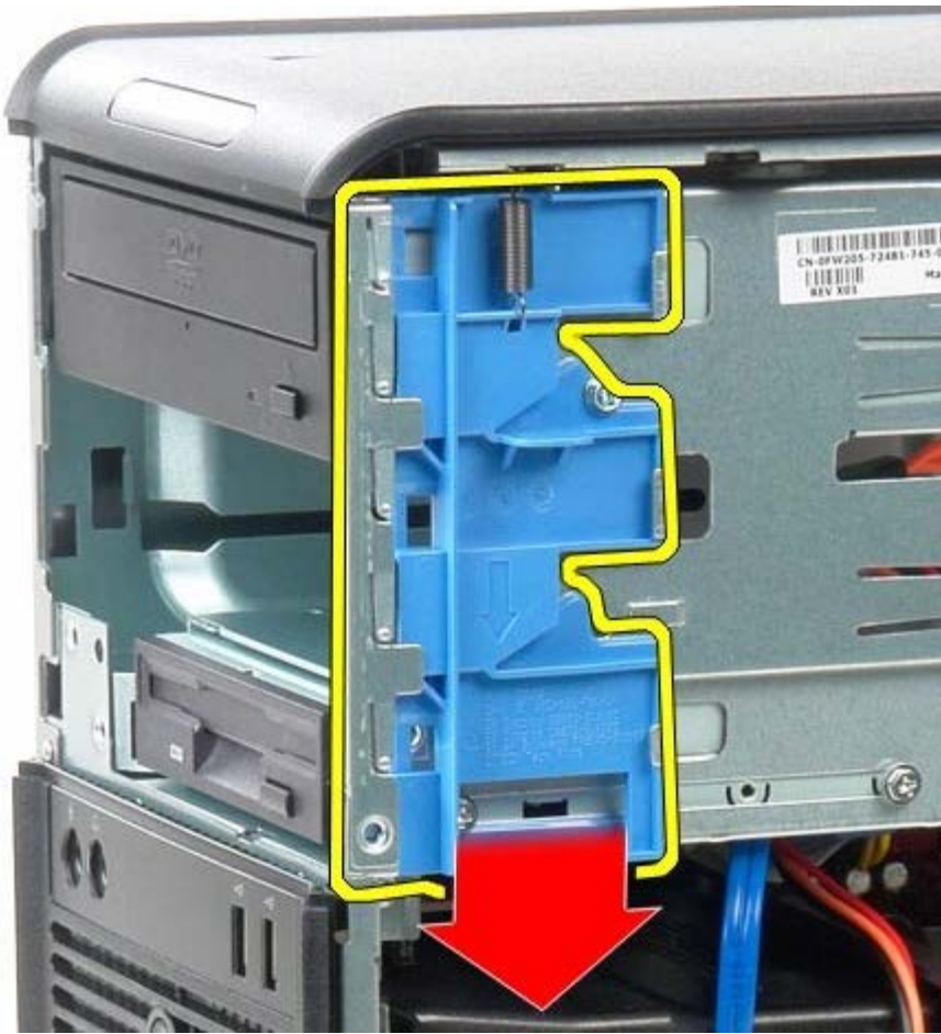
6. Slide the optical drive out of the system.
