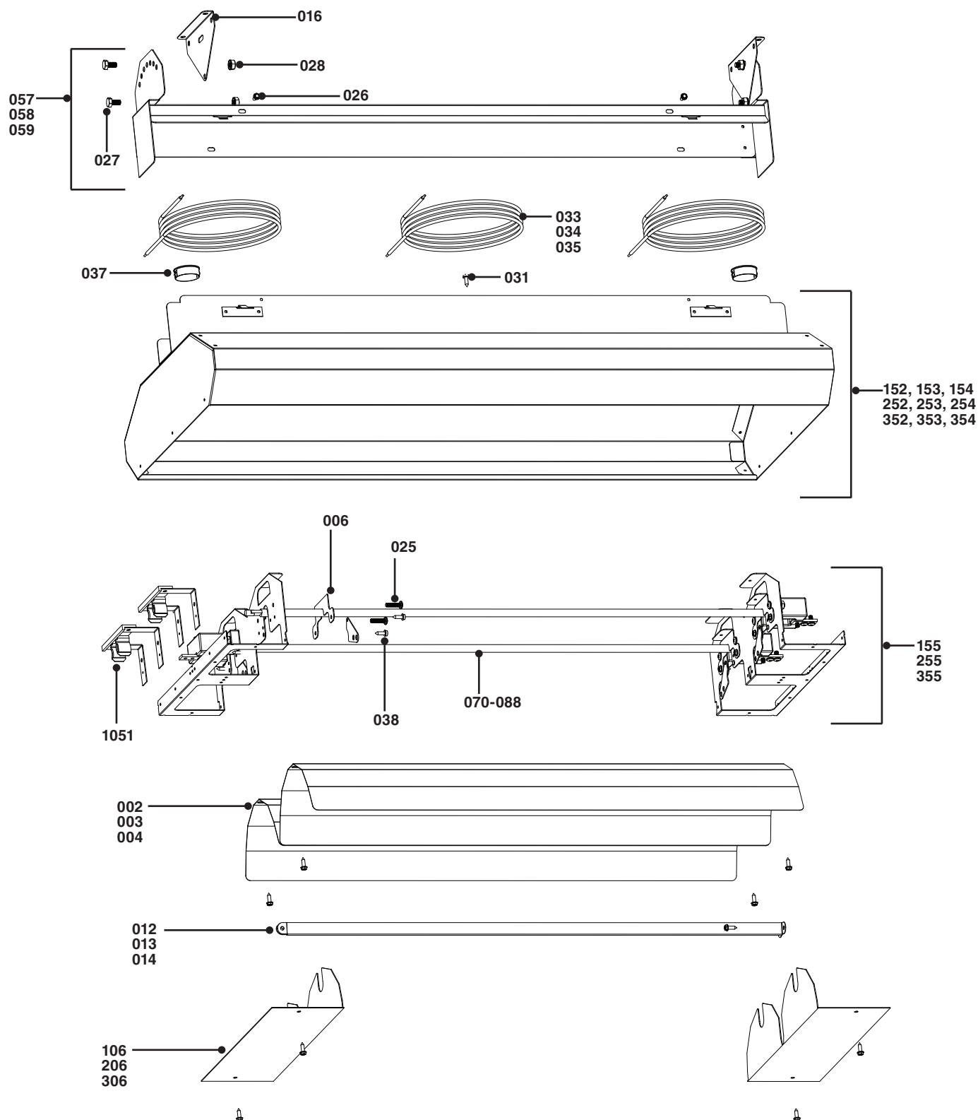
Figure 3.1 • Components
