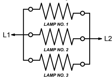
Figure 2.9 • SW Wiring Diagram • Units with 3 Lamps
