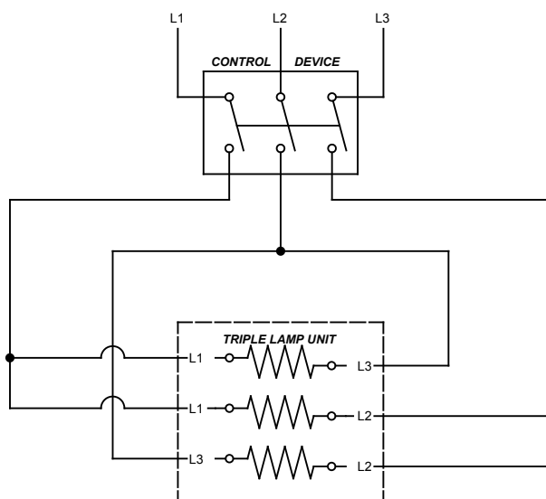
Figure 2.11 • Three Phase Service
