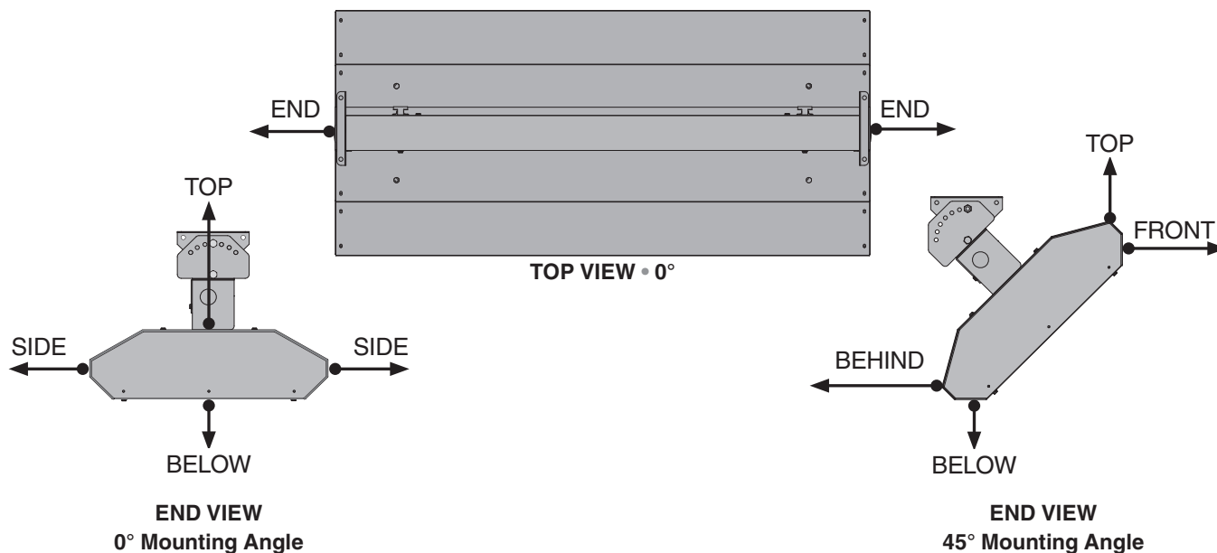
Figure 1.1 • Clearance to Combustibles
