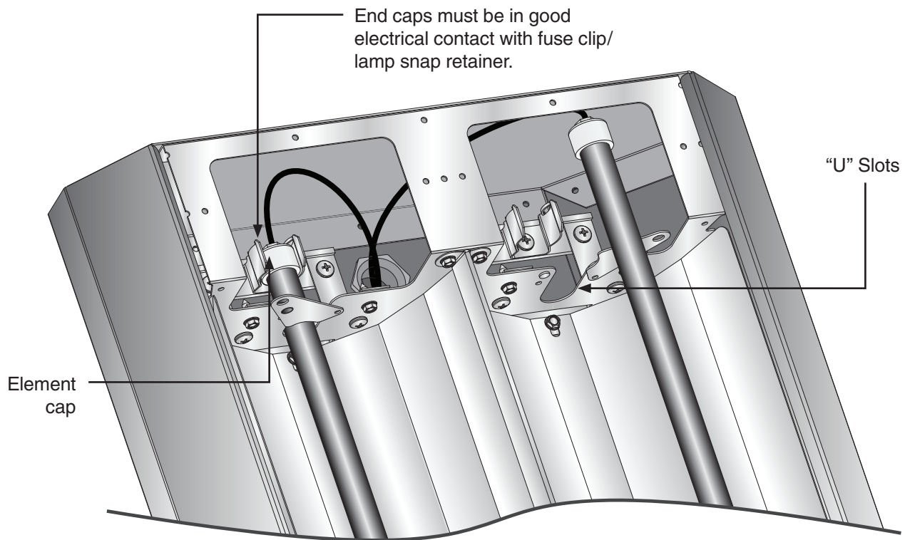
Figure 2.5 • Lamp Installation
