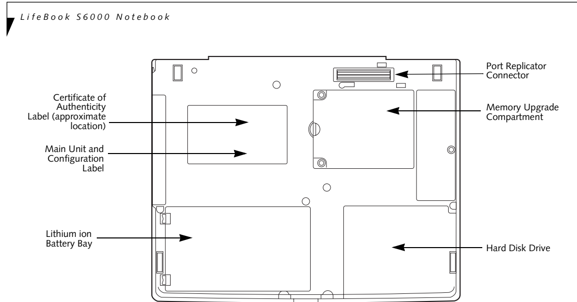
Figure 2-8. LifeBook notebook bottom panel
