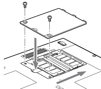
Figure 4-10. Replacing the Memory Compartment Cover
