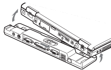
Figure 4-15. Detaching the Port Replicator
