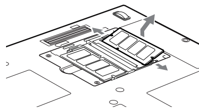
Figure 4-11. Removing a Memory Upgrade Module
