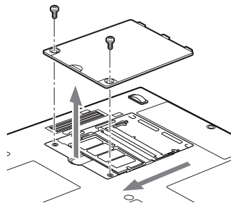
Figure 4-8. Opening the Memory Upgrade Compartment
