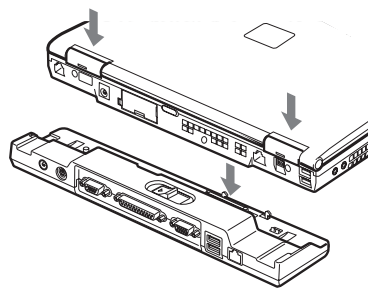
Figure 4-14. Attaching the Port Replicator
