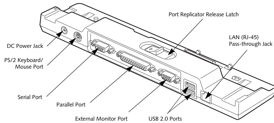
Figure 4-12. Port Replicator back panel
