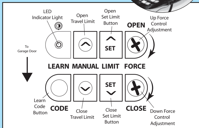
FIG. 6-1 Limit controls.
