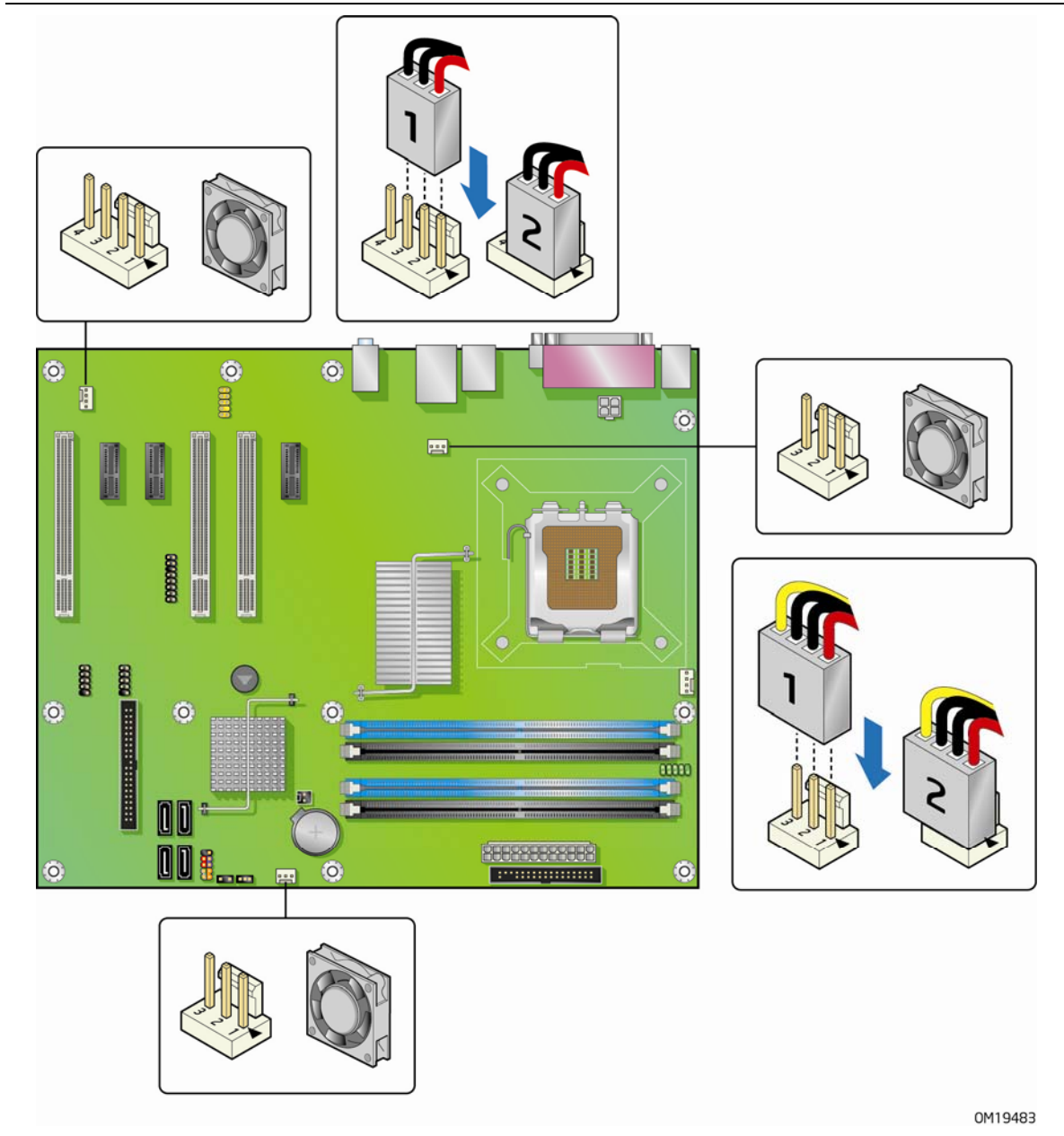
Figure 22. Location of Chassis Fan Headers
