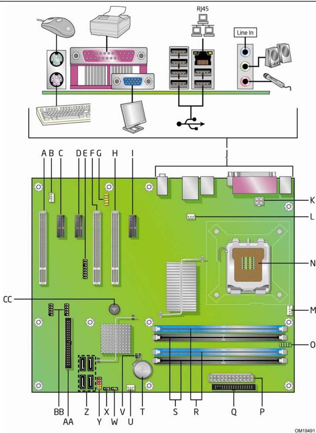
Figure 1. Desktop Board DQ963FX Components
