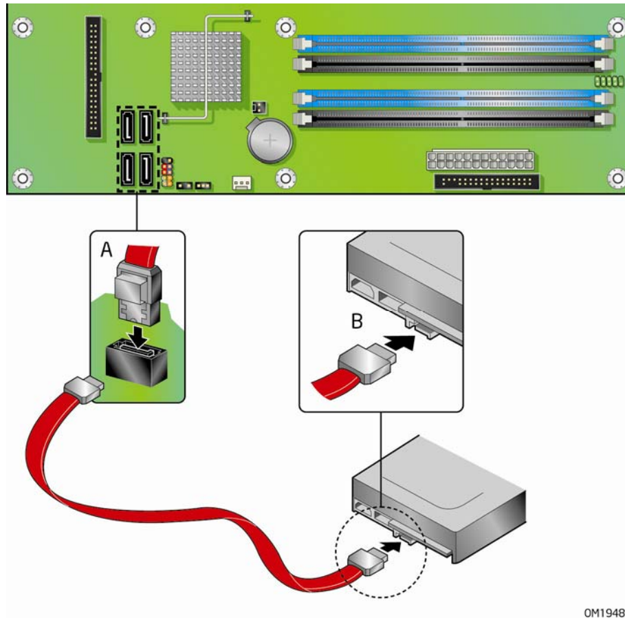
Figure 19. Connecting the Serial ATA Cable
