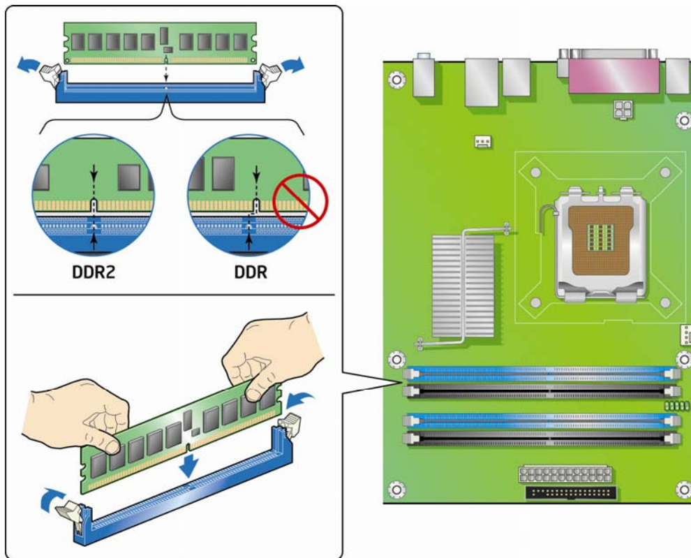
Figure 17. Installing a DIMM
