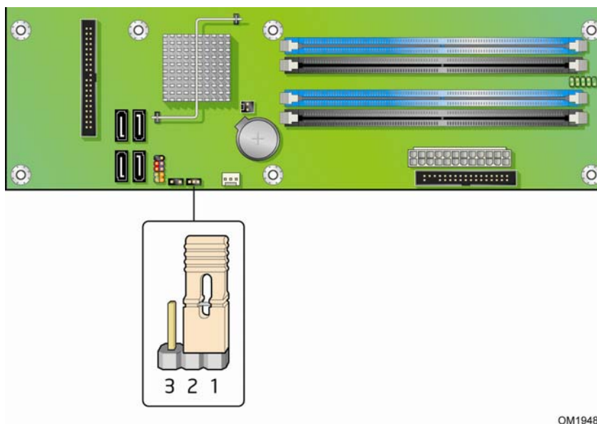
Figure 25. Location of the BIOS Configuration Jumper Block
