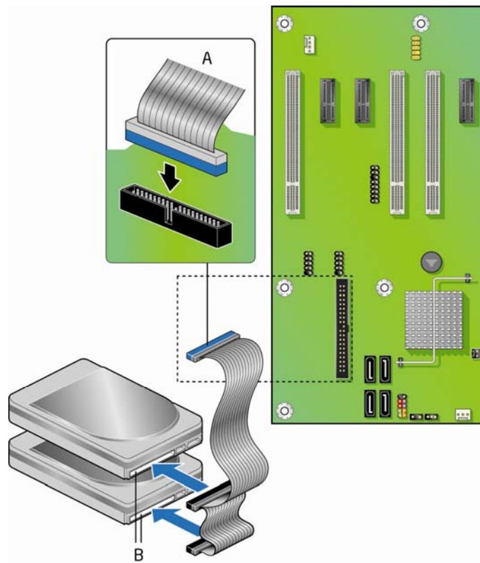
Figure 18. Connecting the IDE Cable
