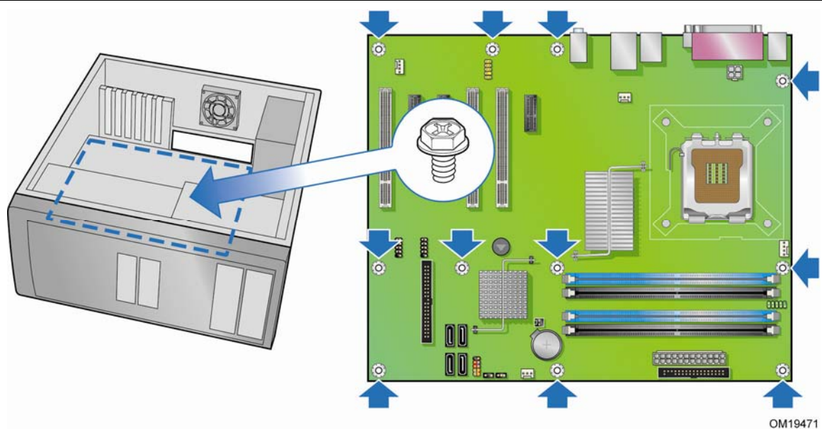
Figure 5. Desktop Board DQ963FX Mounting Screw Hole Locations
