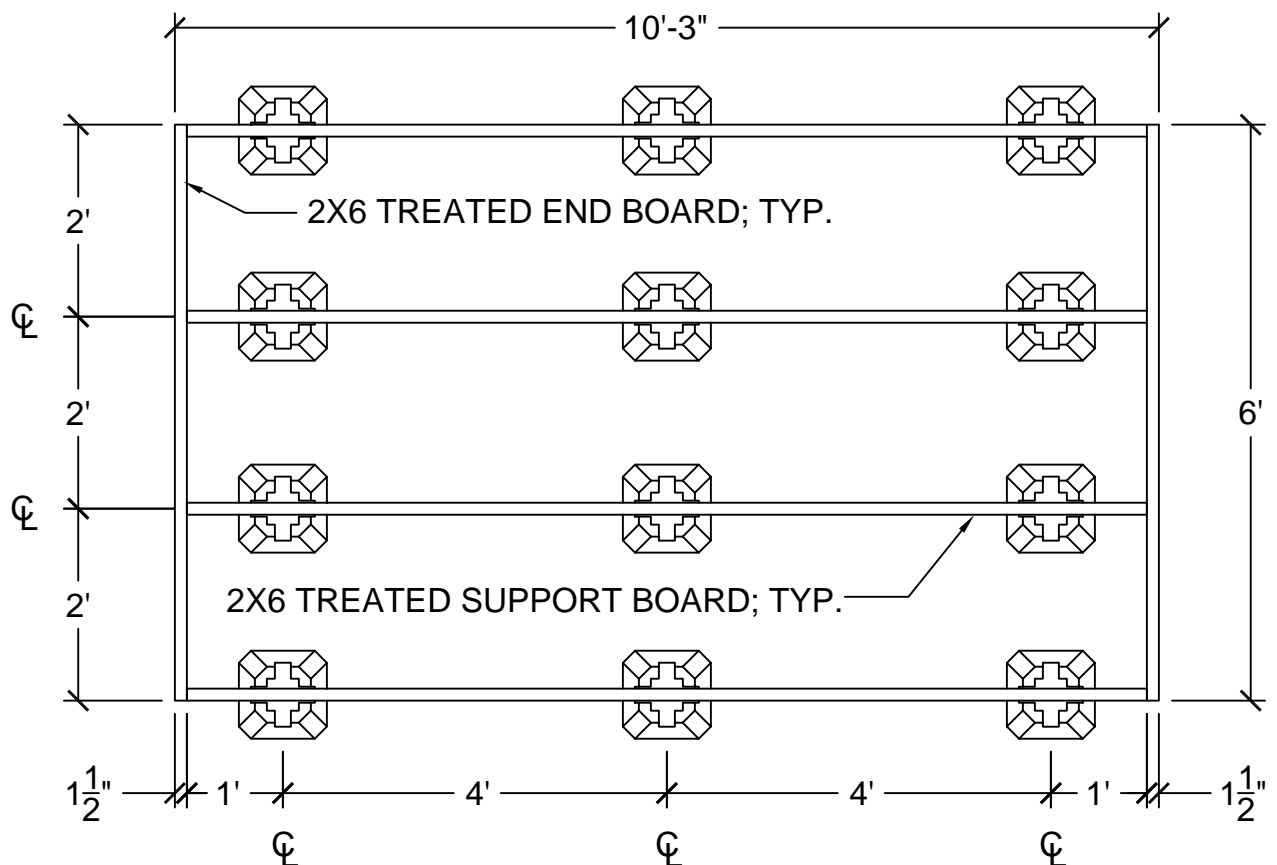
2 FRAMING PLAN SCALE: 1/2" = 1' - 0"
