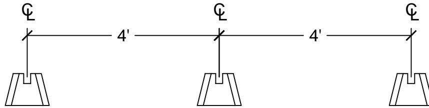
1 DEK-BLOCK LAYOUT SECTION SCALE: 1/2" = 1' - 0"
