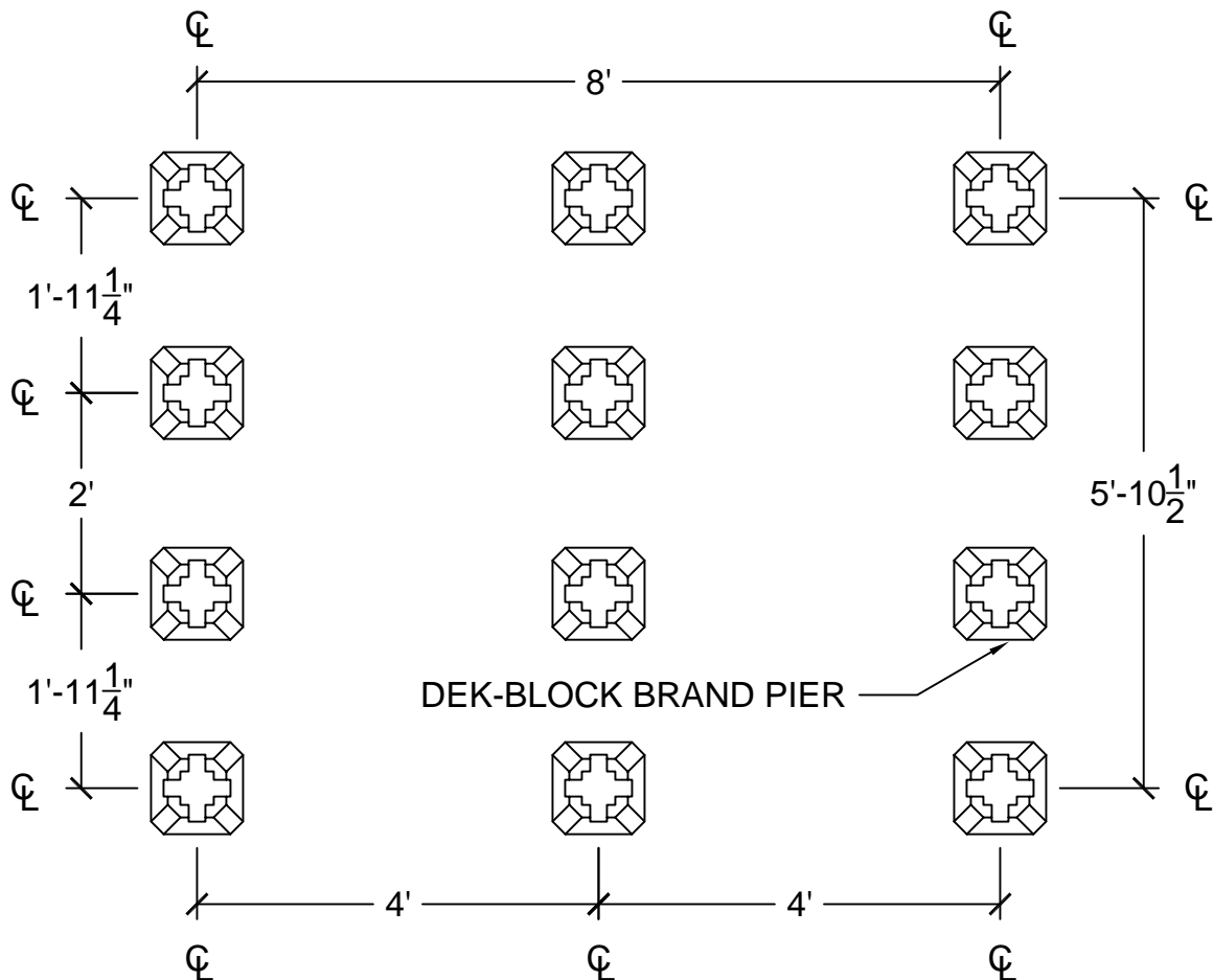
2 DEK-BLOCK LAYOUT PLAN SCALE: 1/2" = 1' - 0"
