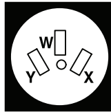
3-wire wall receptacle (10-50R) Figure 5B
