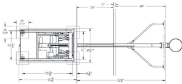
ARENA® BACKSTOP - 10' 8" EXTENSION FOOTPRINT
