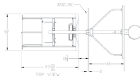
G5 PORTABLE - 5' EXTENSION FOOTPRINT
