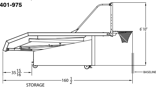
G8 PORTABLE BACKSTOP storage dimensions: 160 1/2" long x 6' 10" high x 76" wide
