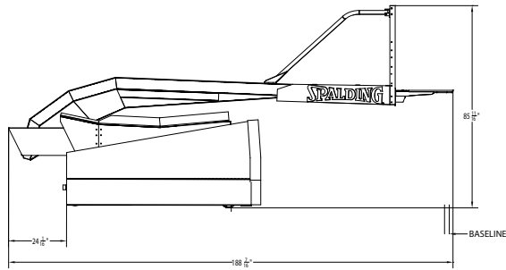
ARENA® BACKSTOP - SPRING ASSIST storage dimensions: 188 7/16" long x 85 11/16" high x 76" wide
