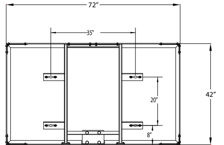
413-019 SuperGlass™ Conversionsb Backboard 72" x 42"
