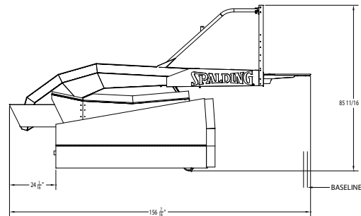
ARENA® BACKSTOP - ELECTRIC storage dimensions: 156 7/16" long x 85 11/16" high x 76" wide
