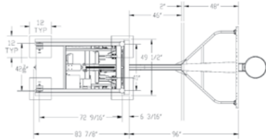
ARENA® BACKSTOP - 8' EXTENSION FOOTPRINT
