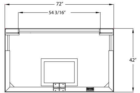
413-001 SuperGlass™ Prosb Backboard 72" x 42"
