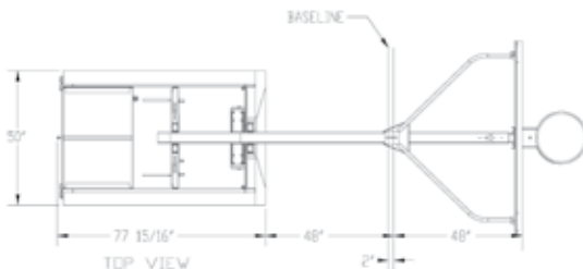
G8 PORTABLE - 8' EXTENSION FOOTPRINT
