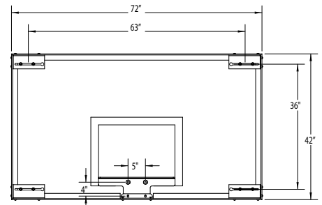
413-007 SuperGlass™ Collegiatesb Backboard 72" x 42"
