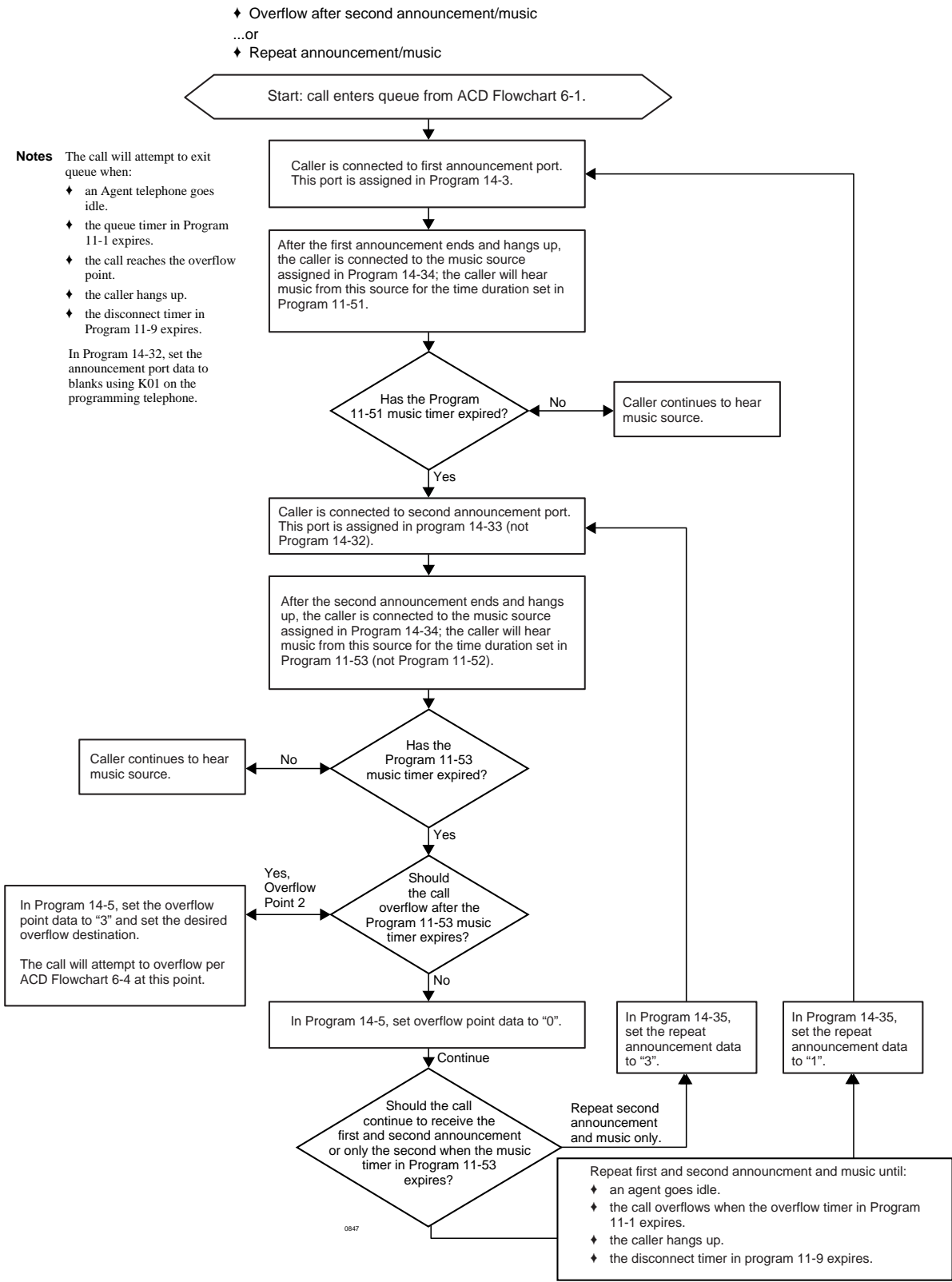
Flowchart 6-9 ACD Queue Pattern Configuration – Two Announcements
